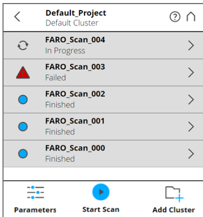
Figure 7-7 List Page
