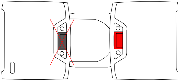
Figure 4-8 : Accessory bay for the status indicator with covers removed
