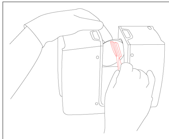
Figure 8-9 Cleaning mirror module with pad and optics cleaning fluid
