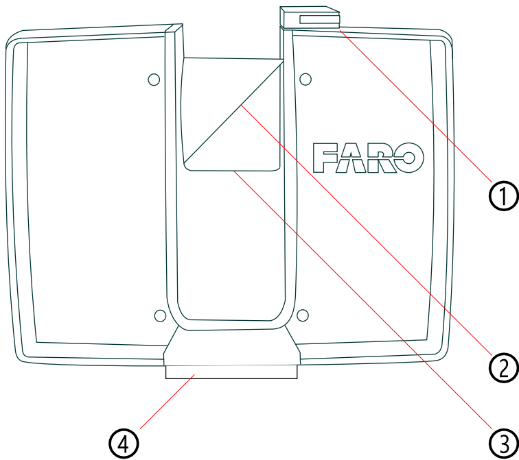
Figure 4-3 Front View of the Focus Premium and Focus Core
